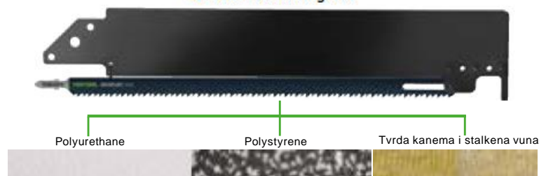
Cross-set cutting set
